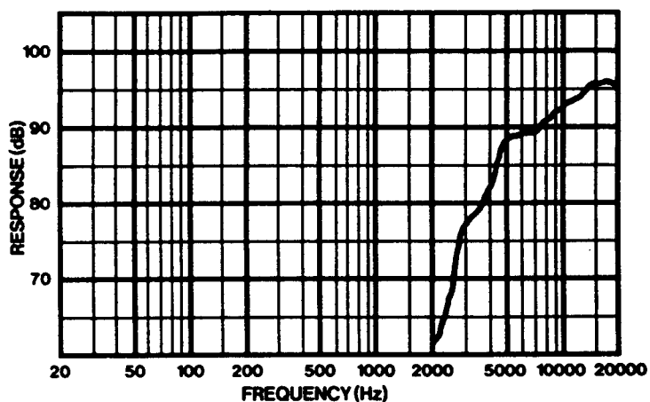
FREQUENCY RESPONSE
